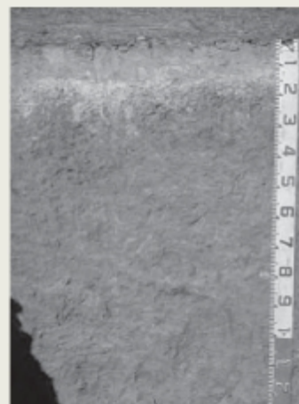
Brown Sodosol
