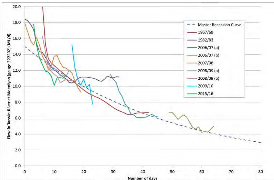
Figure 8-2 Meeniyan base flow master recession curve
