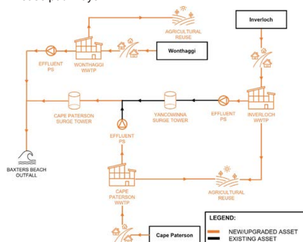
Figure 7-4: Baxters Beach wastewater strategy – infrastructure upgrades overview
