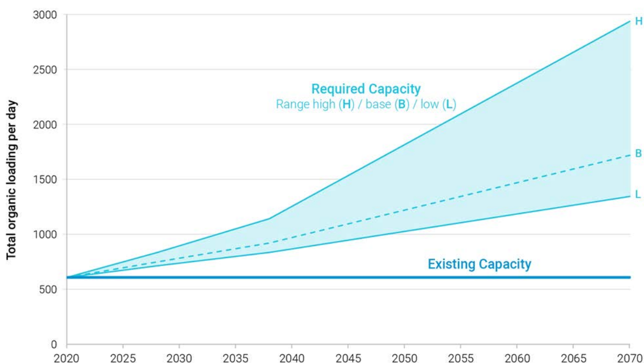
Figure 7-2: Wonthaggi WWTP capacity assessment
