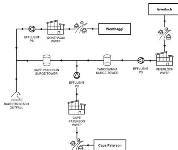
Figure 7-1: Baxters Beach system overview
